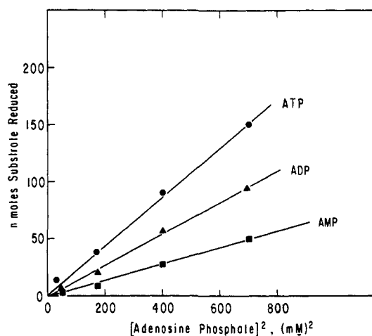
Figure 3. Variation of hydrocarbon product yields with [nucleoside phosphate] 2 for reduction of cyanide by complex 1-BH 4 - in the presence of varying concentrations of AMP, ADP, or ATP. Initial conditions are the same as in Figure 1.
