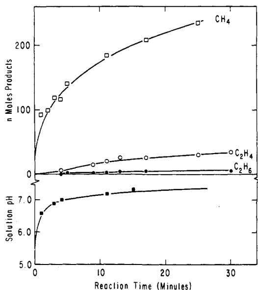
Figure 1. Variation of C 1 - and C 2 -hydrocarbon production, and of solution pH, with reaction time for reduction of cyanide by complex 1-BH 4 - -ATP. Initial concentrations (M): complex 1, 0.019; KCN, 0.025; NaBH 4 , 0.165; ATP, 0.075 in 4.1 ml of 0.2 M, pH 9.6 borate; ATP added prior to BH 4 - addition.
