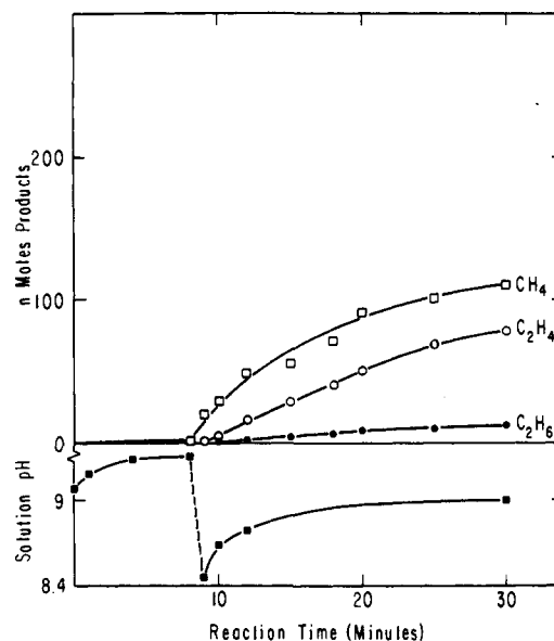
Figure 2. Variation of C 1 - and C 2 -hydrocarbon production, and of solution pH, with reaction time for reduction of cyanide by complex 1-BH 4 - -ATP. Initial conditions the same as in Figure 1, except ATP added after 8 min of reaction time.
